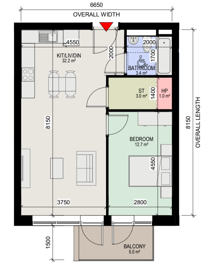
15 Apartment Type 1O 1 : 100
