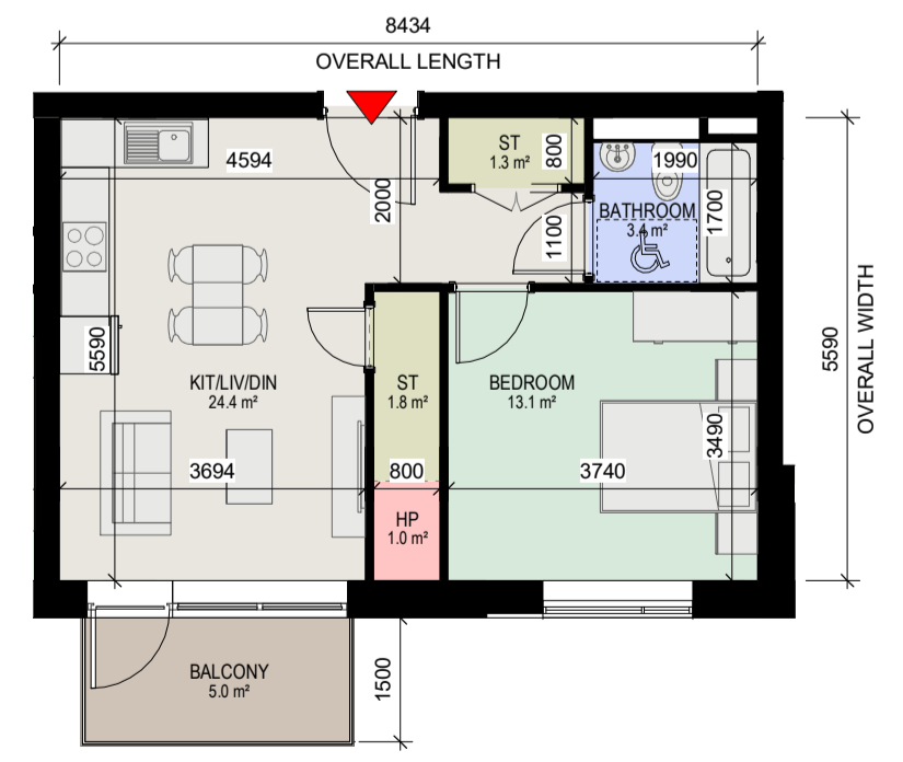
13 Apartment Type 1M 1 : 100
