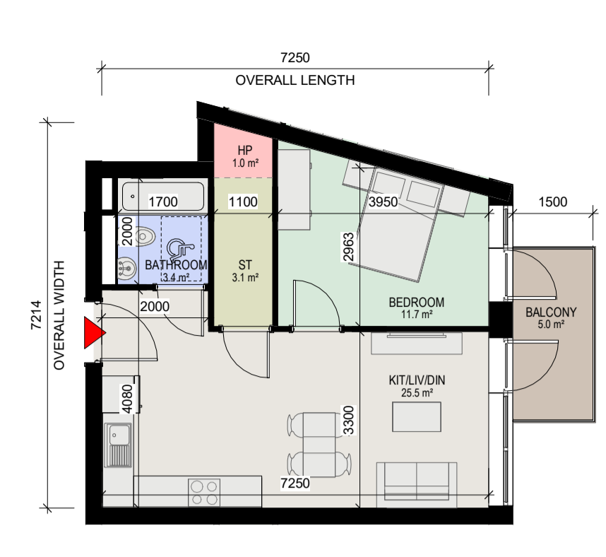
4 Apartment Type 1D 1 : 100
