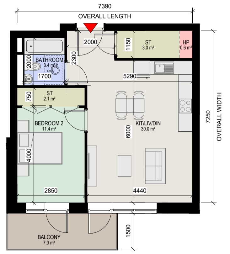
8 Apartment Type 1H 1 : 100
