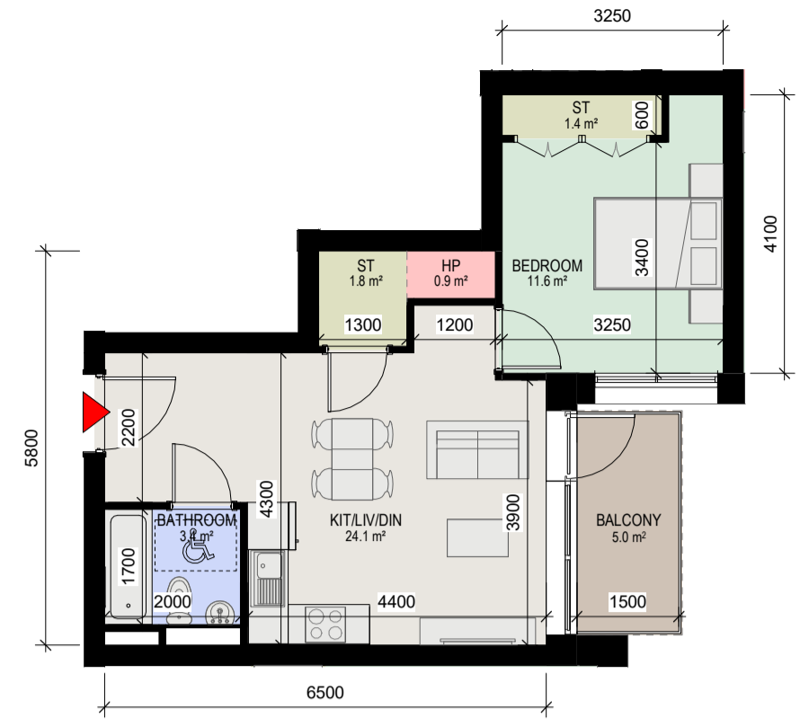
3 Apartment Type 1C 1 : 100
