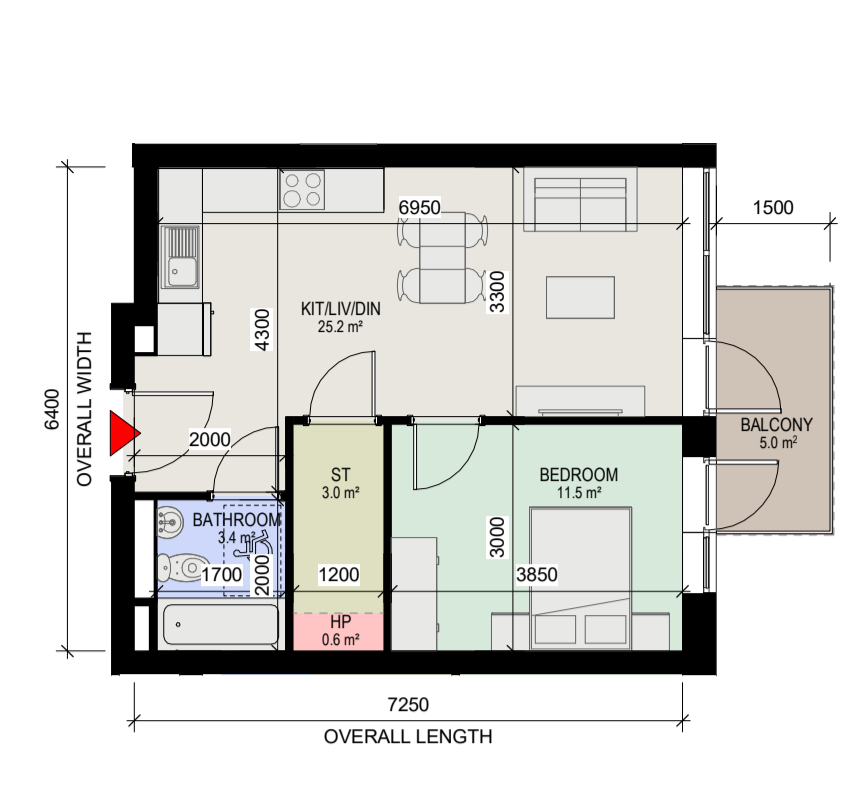
2 Apartment Type 1B 1 : 100
