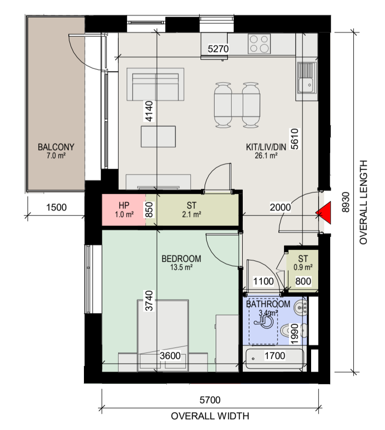
14 Apartment Type 1N 1 : 100
