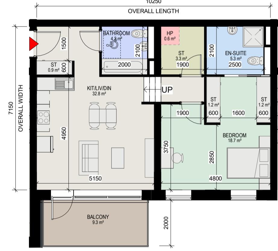
10 Apartment Type 1J 1 : 100
