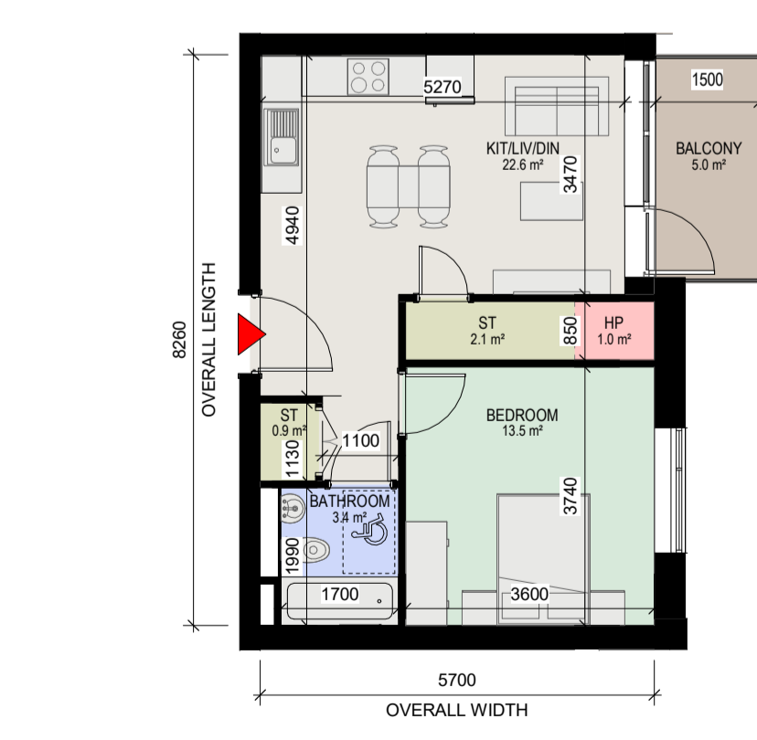
11 Apartment Type 1K 1 : 100
