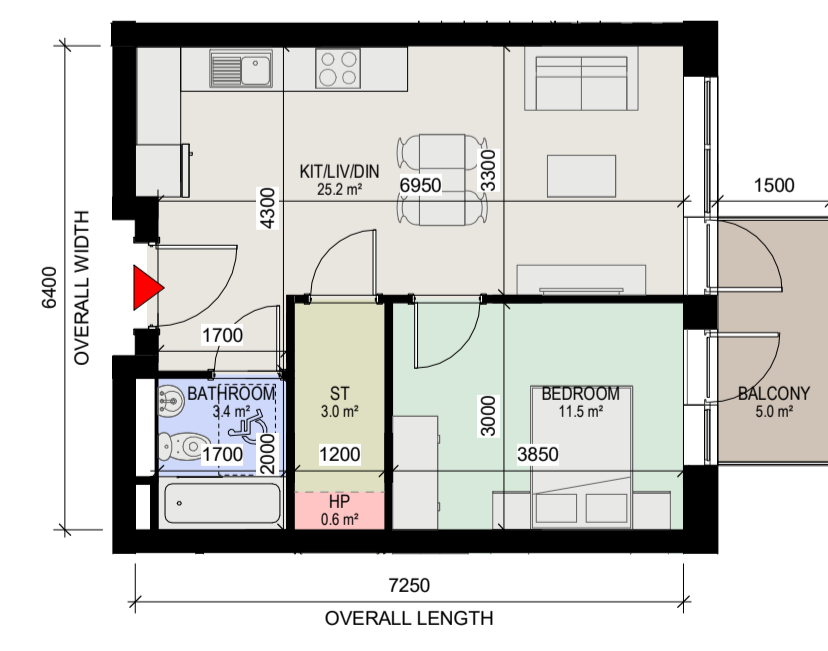
12 Apartment Type 1L 1 : 100
