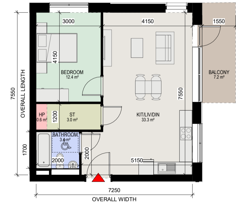
7 Apartment Type 1G 1 : 100
