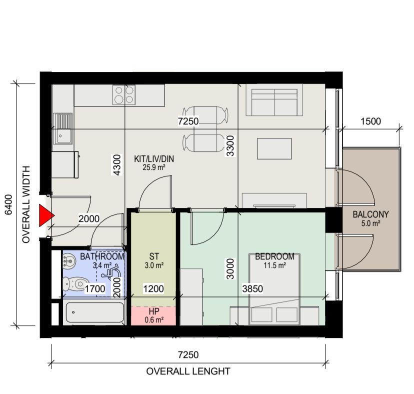
1 Apartment Type 1A 1 : 100
