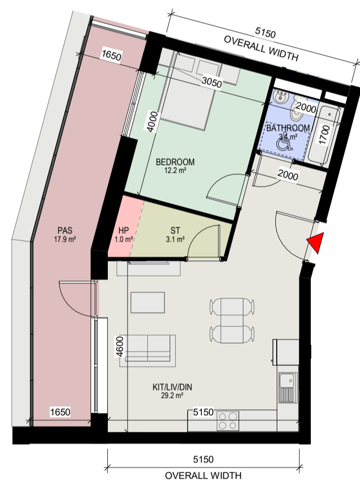
6 Apartment Type 1F 1 : 100
