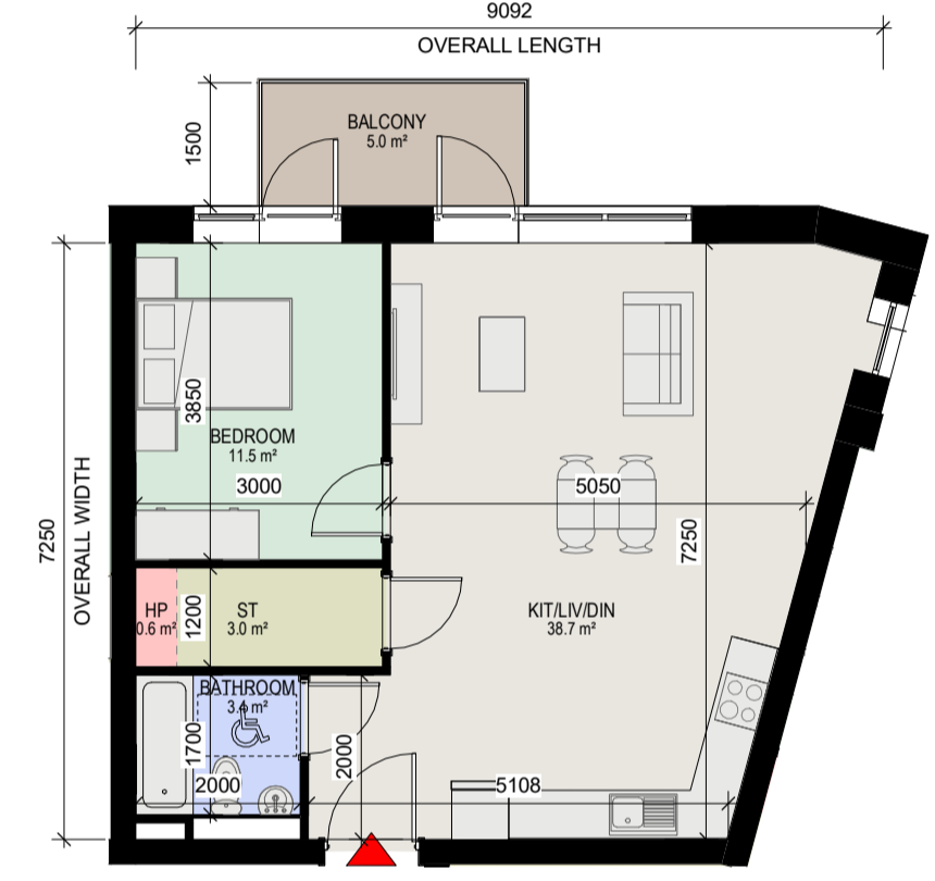
9 Apartment Type 1I 1 : 100
